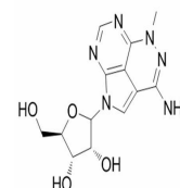
Chemical structure of Triciribine
