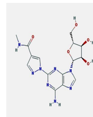
Chemical structure of Regadenoson
