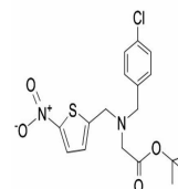
Chemical structure of GSK4112
