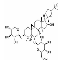
Chemical structure of Astragaloside A
