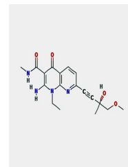
Chemical structure of SAR131675
