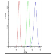
Flow Cytometry analysis of PC-3 cells us...
