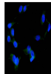
IF analysis of ERp57 using anti-ERp57 an...
