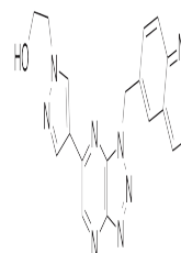
Chemical structure of PF-04217903
