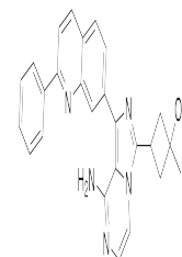
Chemical structure of OSI-906
