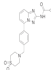
Chemical structure of GLPG-0634
