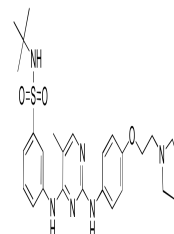
Chemical structure of TG101348
