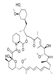
Chemical structure of Rapamycin
