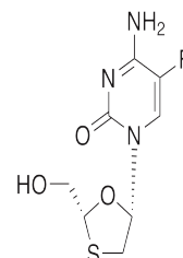
Chemical structure of Emtricitabine
