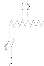
Chemical structure of 8-Gingerol
