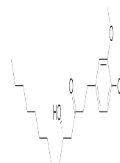
Chemical structure of 10-Gingerol
