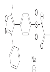
Chemical structure of Parecoxib Sodium
