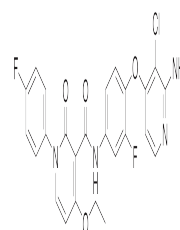
Chemical structure of BMS-777607
