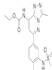
Chemical structure of Bromosporine
