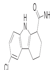
Chemical structure of EX-527
