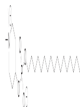
Chemical structure of Perifosine
