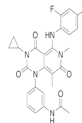
Chemical structure of GSK-1120212
