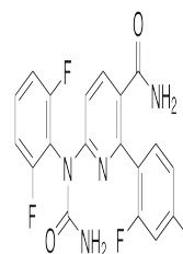
Chemical structure of VX-702
