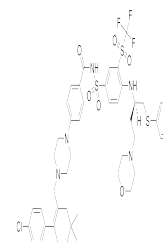
Chemical structure of ABT-263
