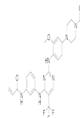
Chemical structure of CO-1686
