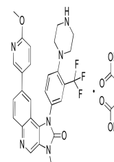
Chemical structure of NVP-BGT226
