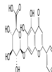
Chemical structure of Baicalin
