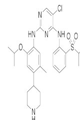
Chemical structure of LDK378
