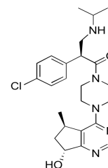
Chemical structure of GDC-0068
