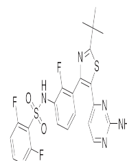
Chemical structure of Dabrafenib
