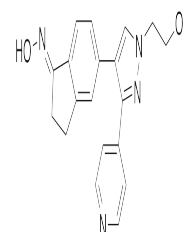
Chemical structure of GDC-0879
