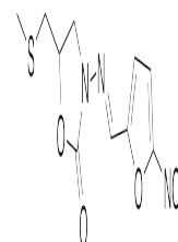
Chemical structure of Nifuratel
