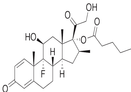
Chemical structure of Betamethasone Valerate
