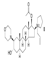
Chemical structure of Rocuronium Bromide
