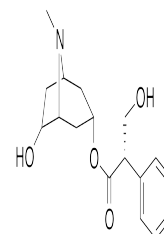
Chemical structure of Anisodamine
