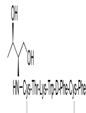
Chemical structure of Octreotide Acetate
