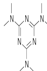
Chemical structure of Altretamine
