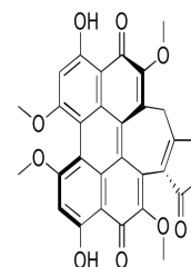
Chemical structure of Hypocrellin B
