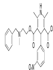
Chemical structure of Nicardipine
