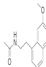
Chemical structure of Agomelatine
