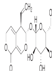
Chemical structure of Gentiopicroside
