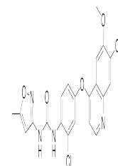
Chemical structure of Tivozanib
