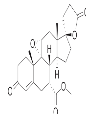
Chemical structure of Eplerenone
