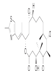
Chemical structure of Epothilone A
