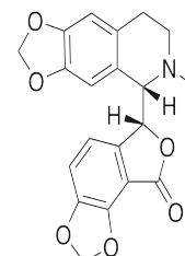
Chemical structure of (+)-Bicuculline
