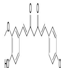
Chemical structure of Demethoxycurcumin
