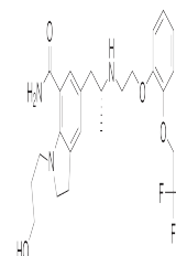
Chemical structure of Silodosin
