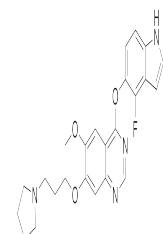
Chemical structure of Cediranib
