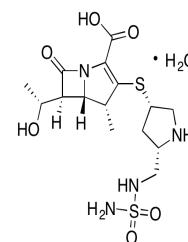
Chemical structure of Doripenem Hydrate
