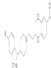
Chemical structure of Iloperidone
