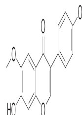
Chemical structure of Glycitein
