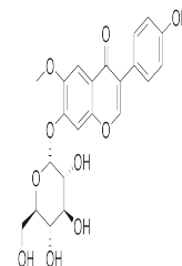
Chemical structure of Glycitin
